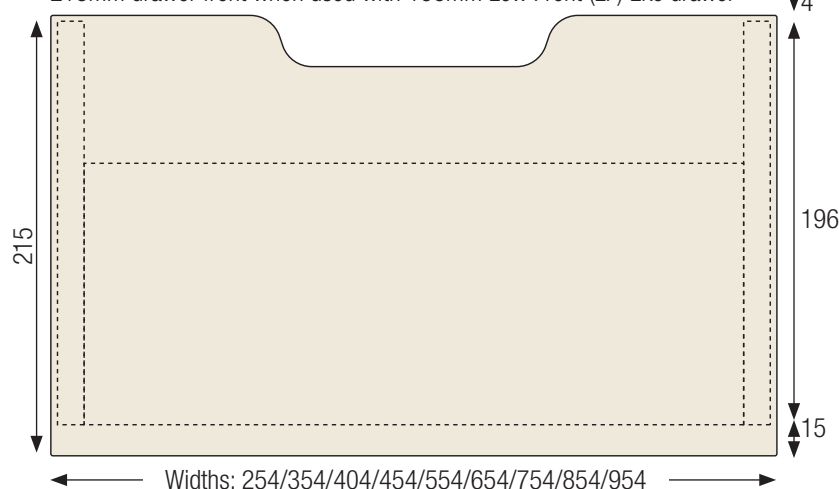
215mm drawer front when used with 196mm Low Front (LF) Eko drawer
