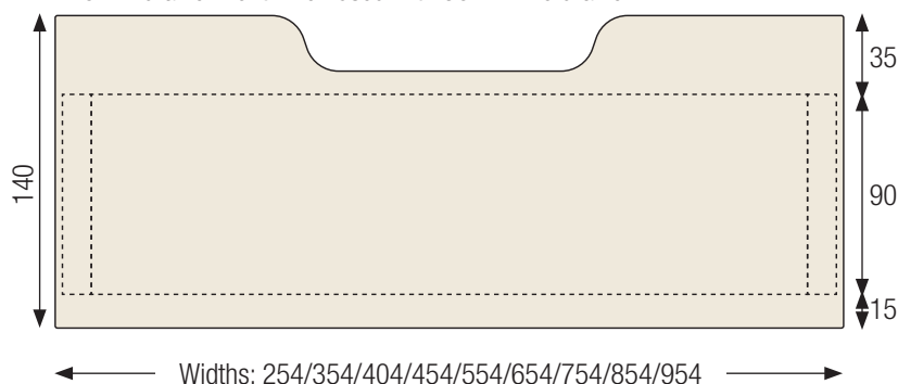
140mm drawer front when used with 90mm Eko drawer
