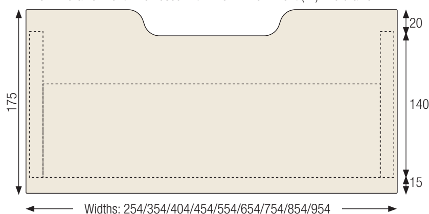
175mm drawer front when used with 140mm Low Front (LF) Eko drawer
